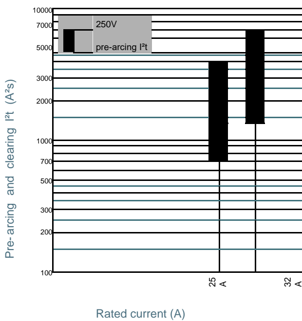
Size 10x38 250V gG with striker
